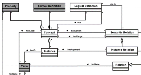
Figure 5. Formal Ontologies
