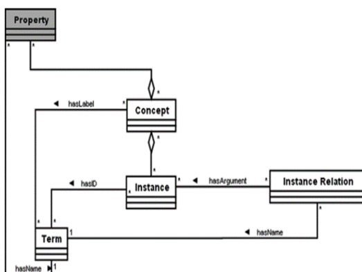
Figure 1. UML Class Diagram for ontology components and its relationship
