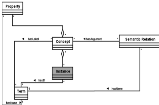
Figure 4. Software Ontology
