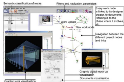
Figure 2. Information Ontology
