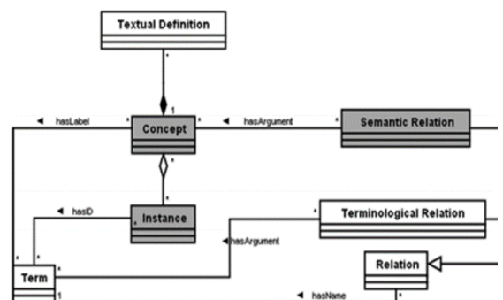
Figure 3. Linguistic Ontology
